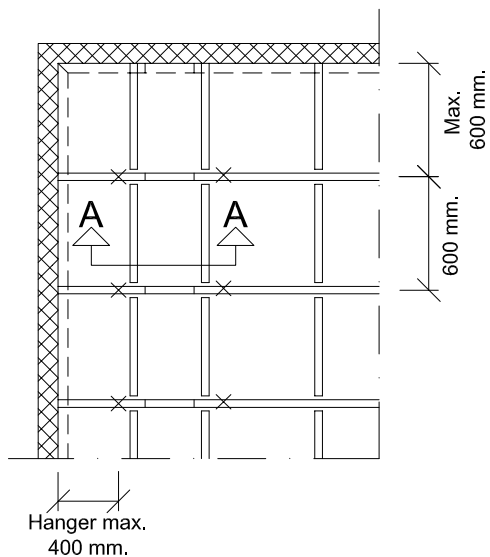
PLAN CUTOUT
