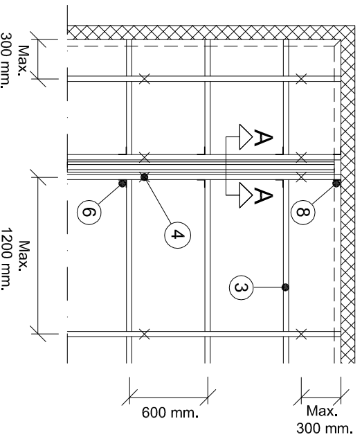
PLAN CUTOUT
