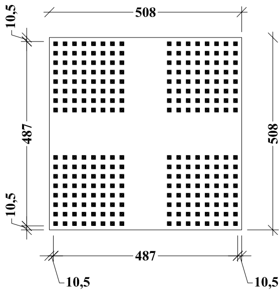
Access Panel Quattro 42 with the measurement of 508 x 508 mm
