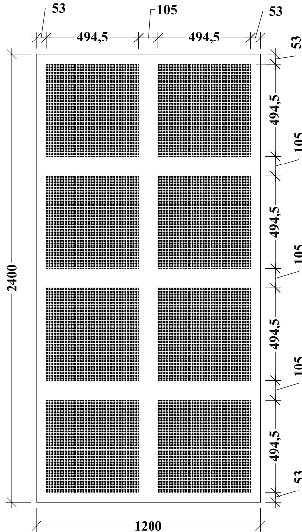
BIG Quattro 71 with the measurement of 1200 x 2400 mm
