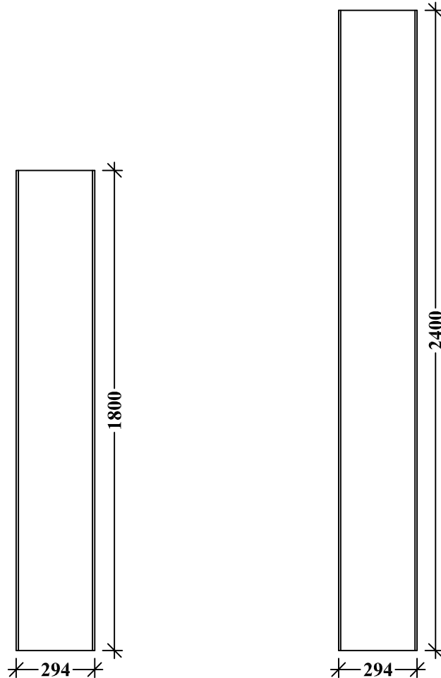
Plank with the modular measurements of 294 x 1800 mm to 294 x 2400 mm
