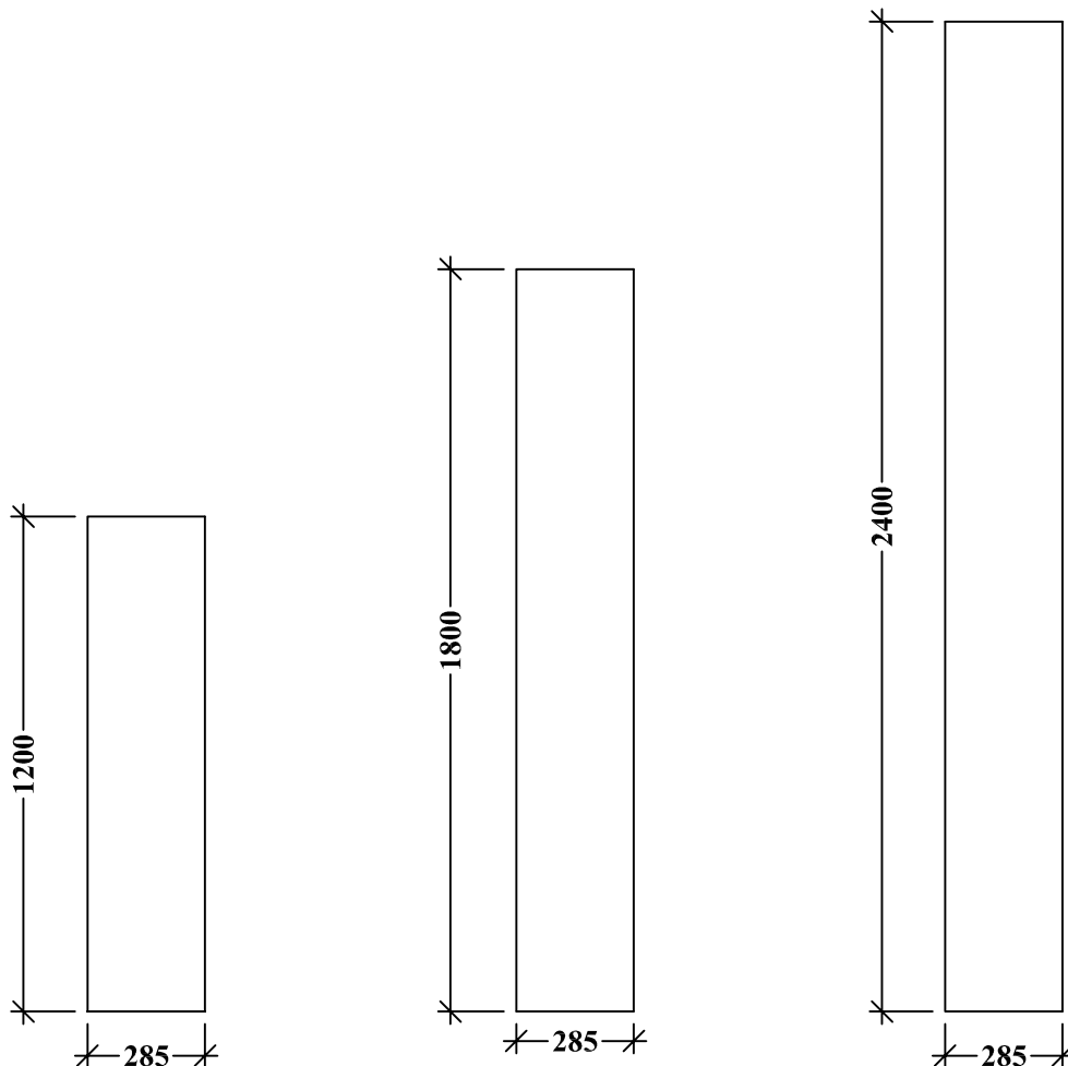
Base 33 with the actual size of 285 x 1200 mm, 285 x 1800 m and 285 x 2400 mm
